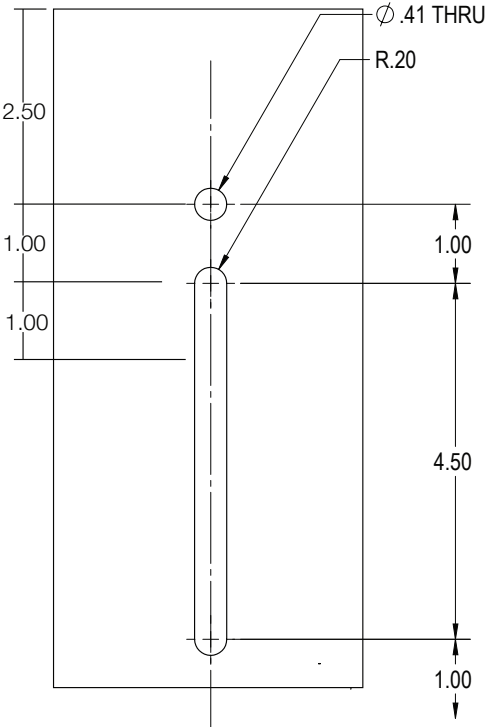
Drilling Template for (UAM)
